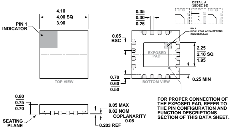
COMPLIANT TO JEDEC STANDARDS MO-220-WGGC. Figure 37. 16-Lead Lead Frame Chip Scale Package [LFCSP] 4 mm x 4 mm Body and 0.75 mm Package Height (CP-16-23) Dimensions shown in millimeters
