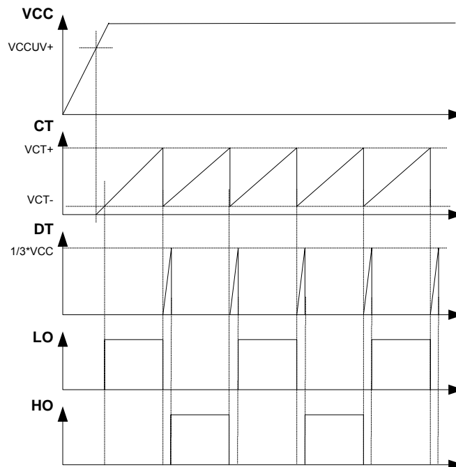
Figure 3: Oscillator waveforms
