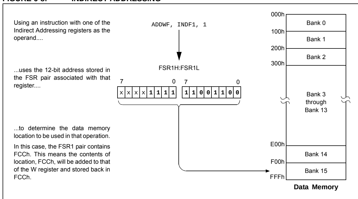
FIGURE 6-8: INDIRECT ADDRESSING
