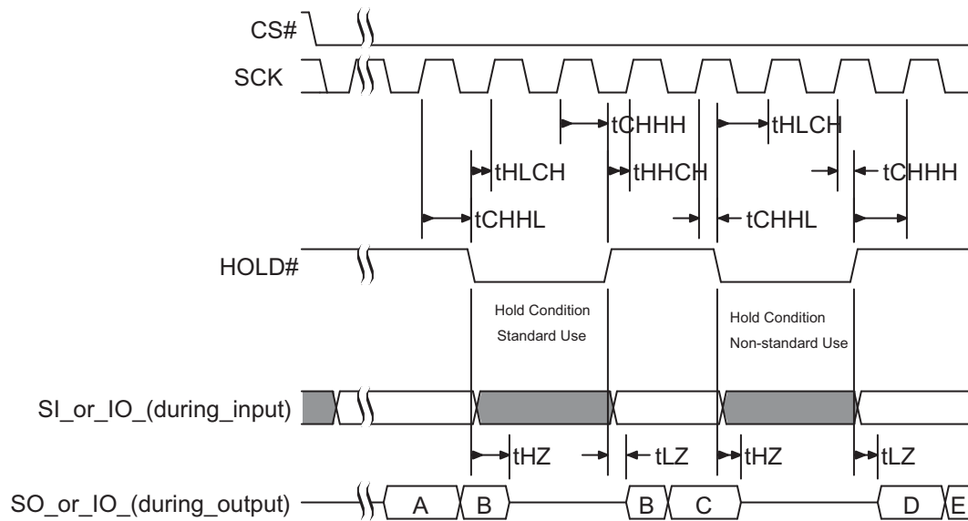
Figure 34. Hold Timing
