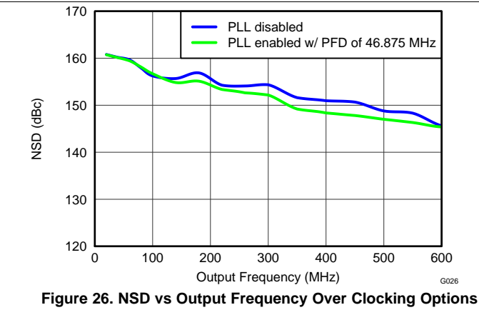
Figure 26. NSD vs Output Frequency Over Clocking Options
