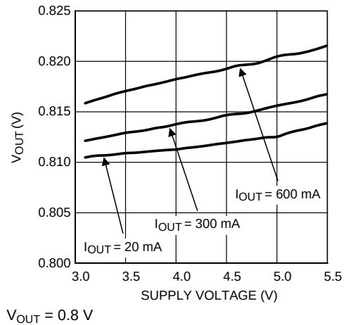
Figure 22. Output Voltage vs Supply Voltage
