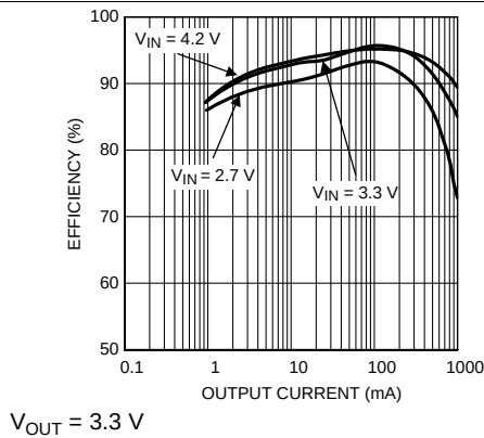
Figure 39. Autmode Efficiency vs I_{LOAD}
