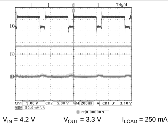
Figure 41. Switch Pins in Buck Mode Operation
