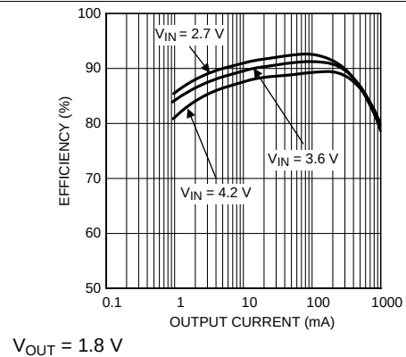
Figure 40. Autmode Efficiency vs I_{LOAD}
