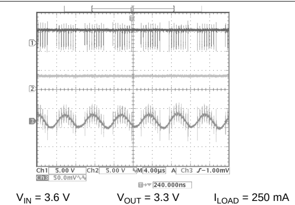
Figure 42. Switch Pin on Edge of Buck Mode Operation
