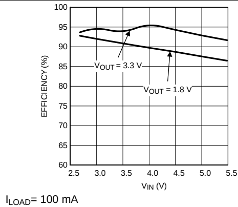
Figure 37. Efficiency vs VIN
