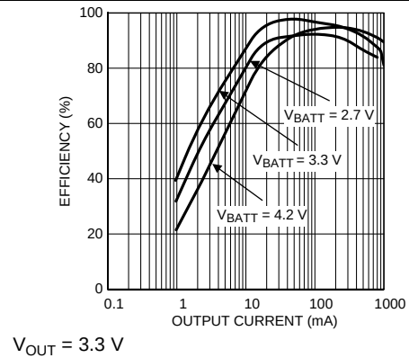
Figure 38. Forced PWM Efficiency vs I_{LOAD}
