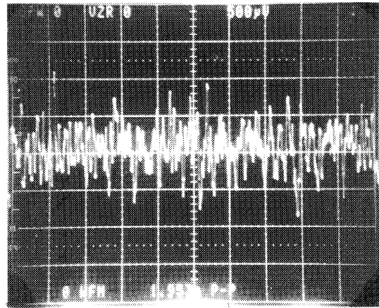
FIGURE 18. PEAK-TO-PEAK NOISE VOLTAGE (0.1Hz TO 10Hz) A_{\text{CL}} = 25,000\text{V/V} Horizontal Scale = 1s/Div. Vertical Scale = 0.002\mu\text{V/Div.} , E_N = 0.08\mu\text{V}_{\text{P-P RTI}}
