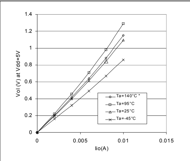
Figure 99. Typical V_{OL} at V_{DD} = 5V (standard)
