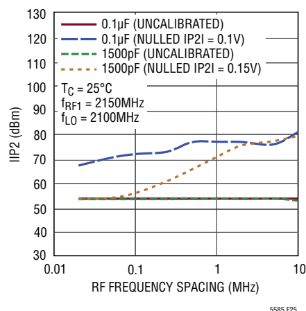
Figure 25. IIP2 vs Common Mode Decoupling Capacitance
