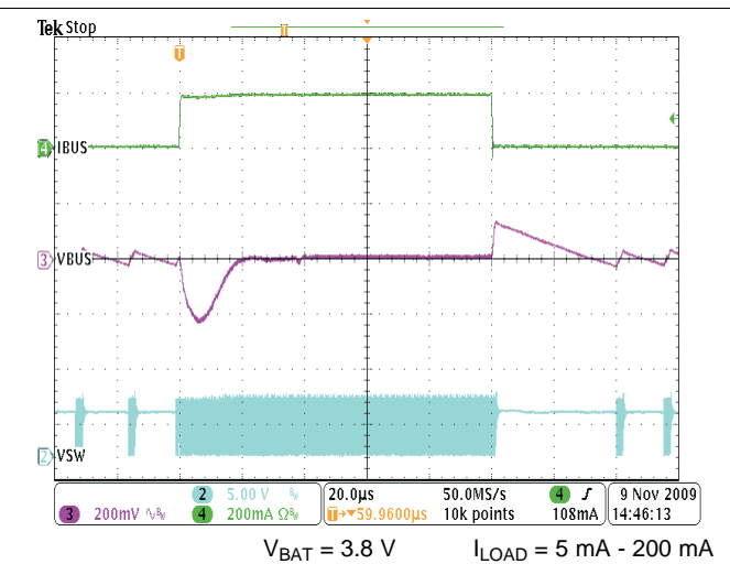
Figure 14. Transient Response
