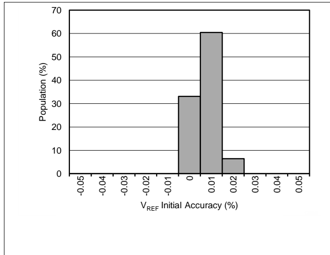
Figure 1. Initial Accuracy Distribution ( V_{REF} )
