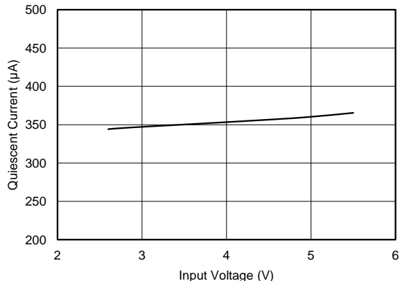
Figure 32. Quiescent Current vs Input Voltage
