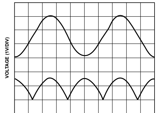
TIME (1ms/DIV)
