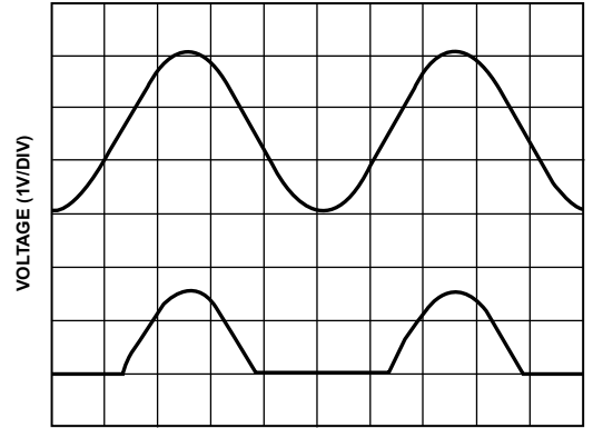
Figure 50. Half-Wave Rectifier Signal (OUT A in Figure 49)
