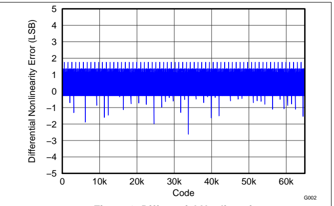
Figure 2. Differential Nonlinearity
