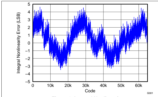
Figure 1. Integral Nonlinearity
