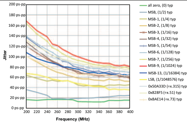
Figure 3. Fractional Divider Bit Selection Impact on Jitter
