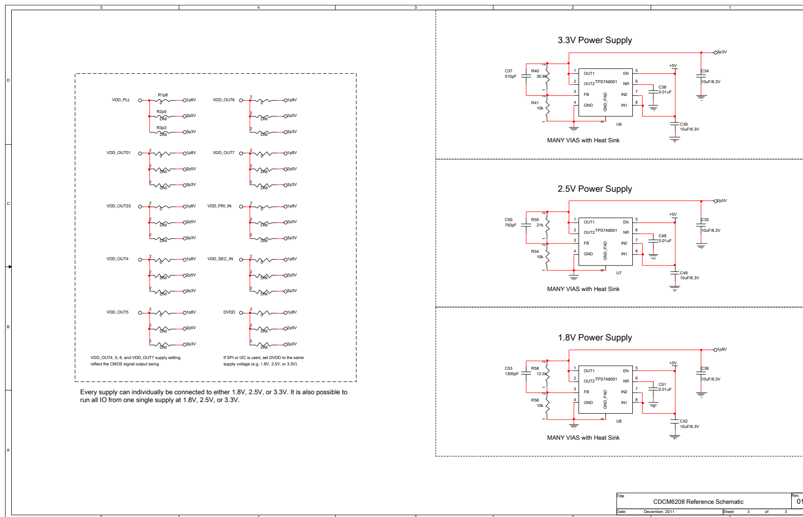
Figure 62. Schematic Page 3
