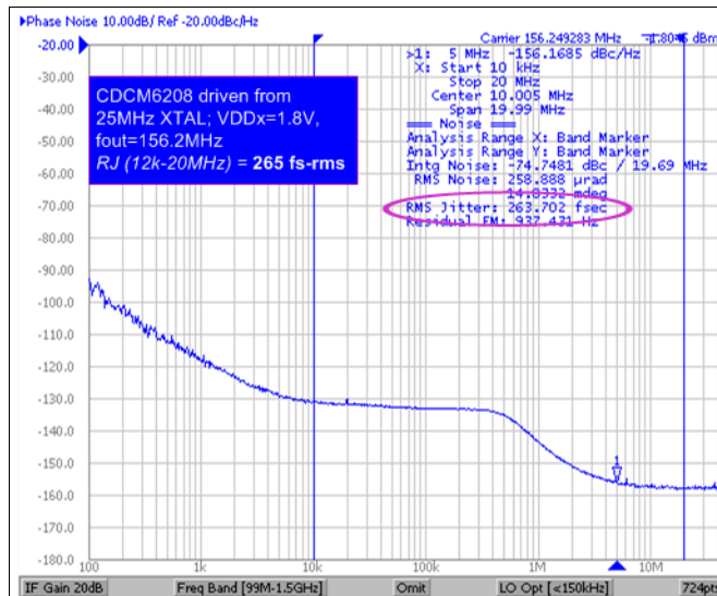
Figure 54. Typical Device Output Phase Noise and Jitter for 25 MHz
