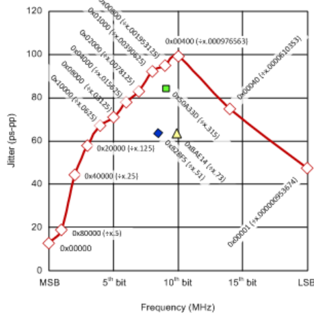
Figure 3. Fractional Divider Bit Selection Impact on Jitter
