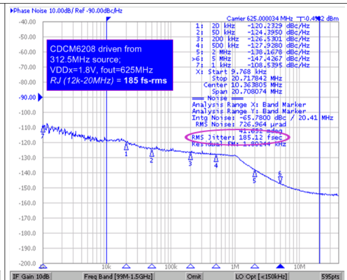
Figure 55. Typical Device Output Phase Noise and Jitter for 312.5 MHz
