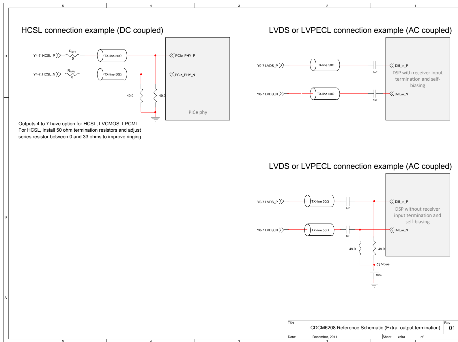
Figure 63. Schematic Page 4
