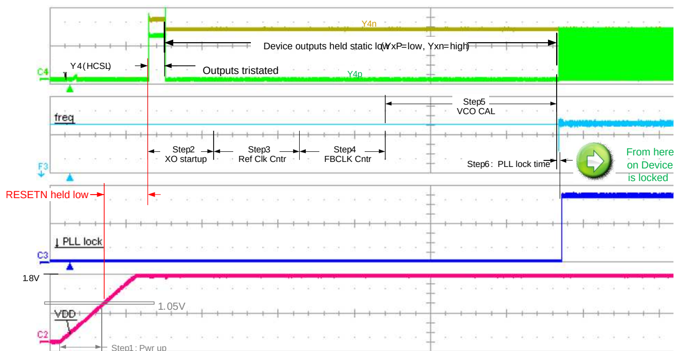
Figure 41. Powerup Time
