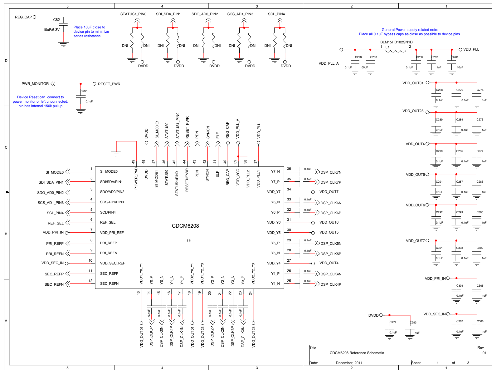
Figure 60. Schematic Page 1
