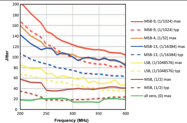
Figure 4. Fractional Divider Input Frequency Impact on Jitter
