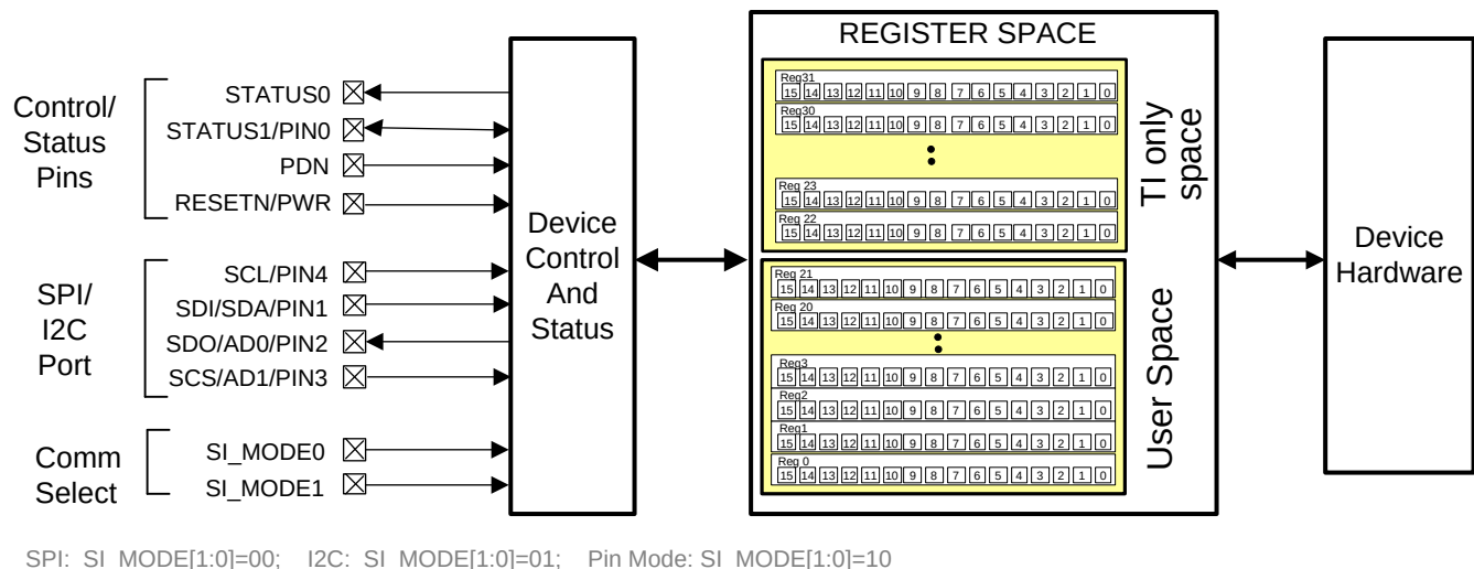
Figure 27. CDCM6208V2G Interface and Control Block
