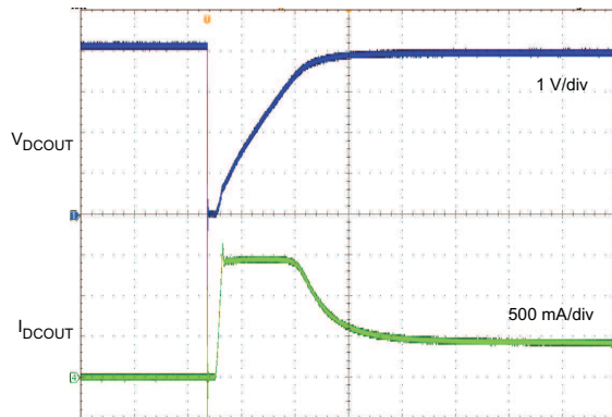
Figure 18. Hotplug 1000µF Capacitor into DCOUT
