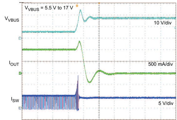
Figure 19. OVP Response
