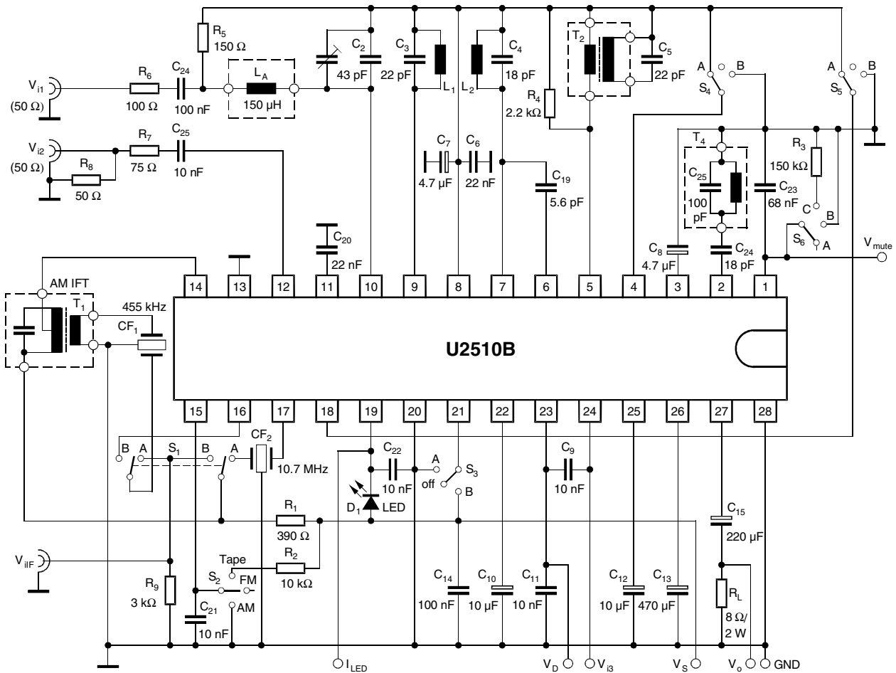
Figure 16. Test Circuit
