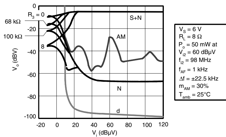
Figure 14. FM Section: Audio Output Level
