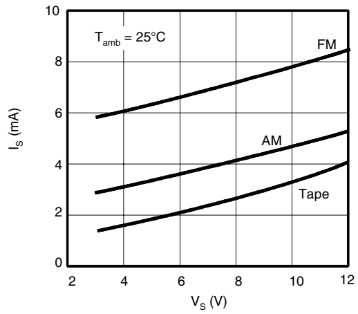
Figure 3. Quiescent Current
