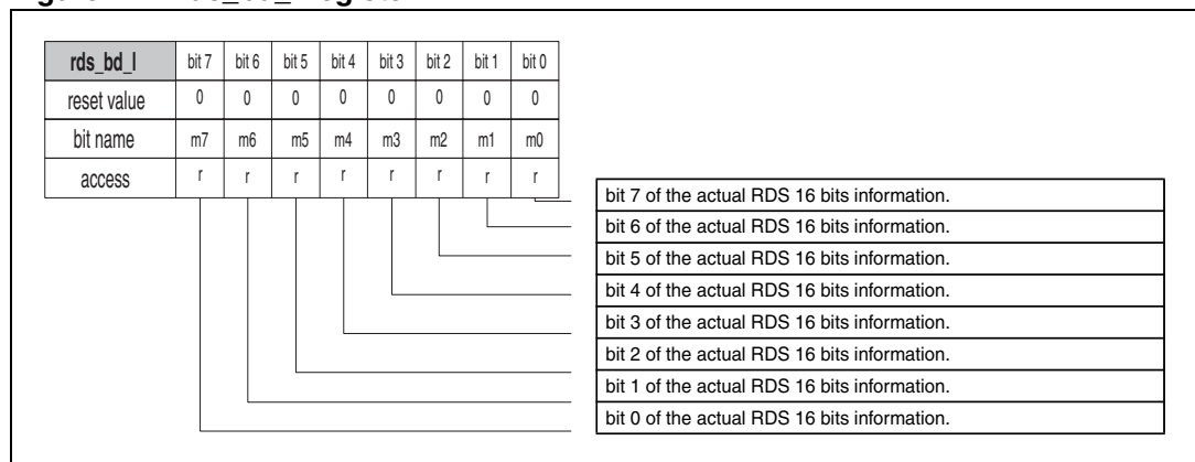
Figure 14. rds_bd_l register
