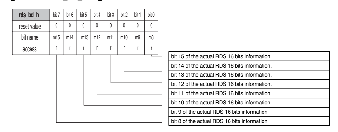
Figure 13. rds_bd_h register
