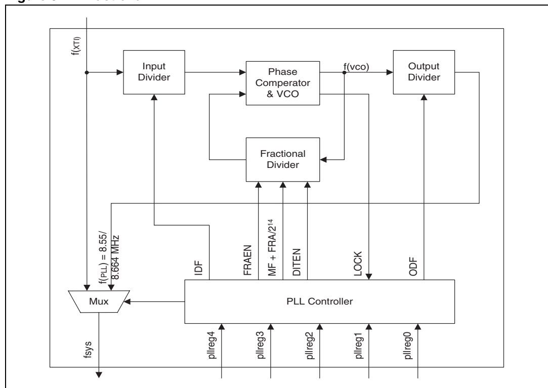
Figure 3. Fractional PLL
