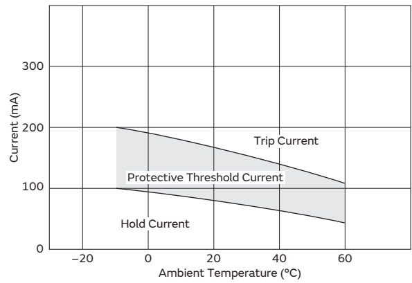
PTGL07BD220N3B51B0
