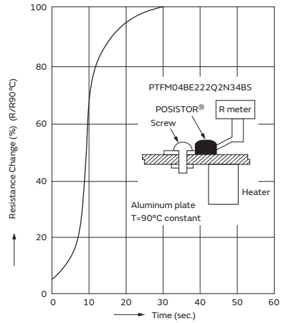
Relation between resistance change and time after POSISTOR® PTFM04BE222Q2N34BS is installed on the part heated at a constant temperature of 90°C (3mm thick aluminum sheet) is shown in the figure above.
