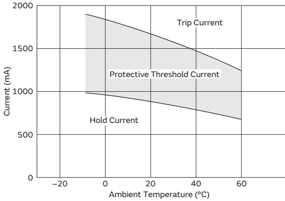
PTGL13AR0R8H2B71B0
