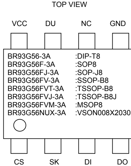
Figure 3. Pin Configuration
