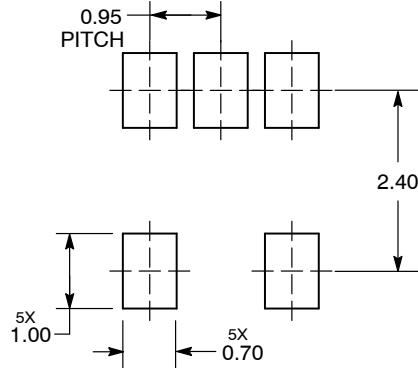
DIMENSIONS: MILLIMETERS
