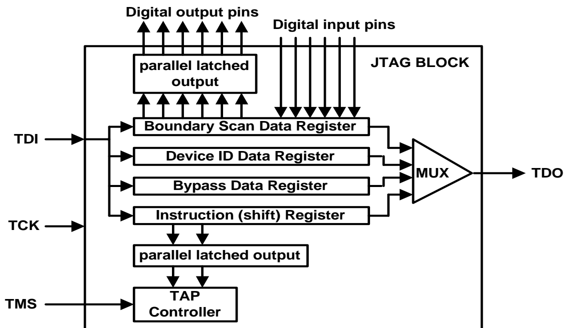
Figure 14. Test Access Port Architecture
