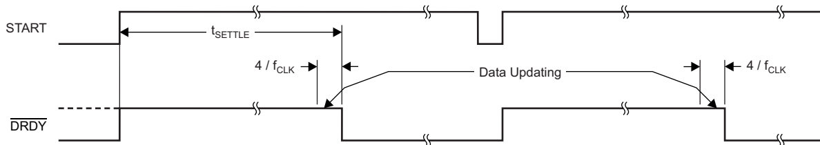
Figure 51. DRDY with No Data Retrieval in Single-Shot Mode
