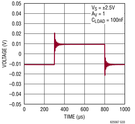
Small-Signal Response
