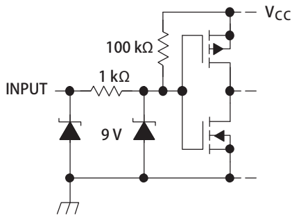
Figure 27. D Input
