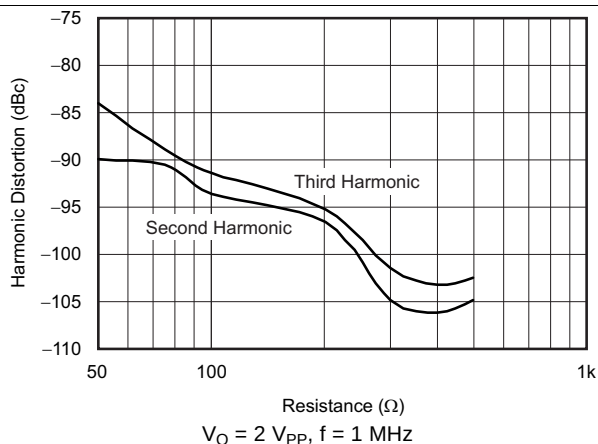
Figure 52. Harmonic Distortion vs Load Resistance
