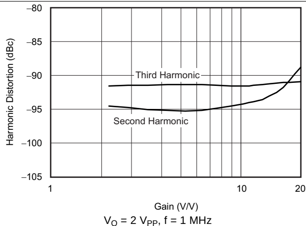
Figure 53. Harmonic Distortion vs Noninverting Gain
