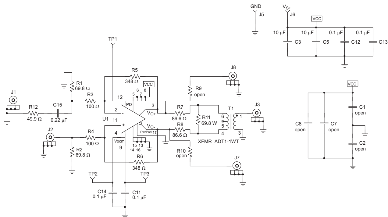
Figure 62. TMS4508 EVAL1 EVM Schematic
