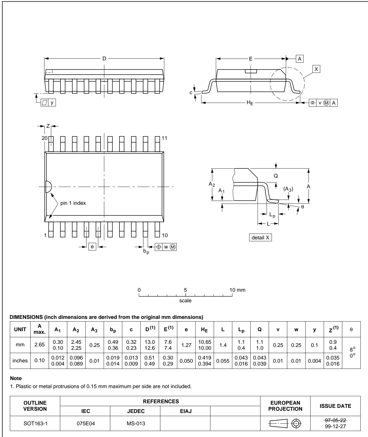
Fig 6. SO20 package outline (SOT163-1).
