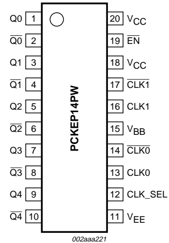
Fig 2. TSSOP20 pin configuration.
