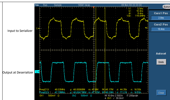
Figure 18. 48 MHz Clock at Serializer and Deserializer
