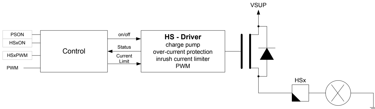
Figure 23. HS Circuitry
