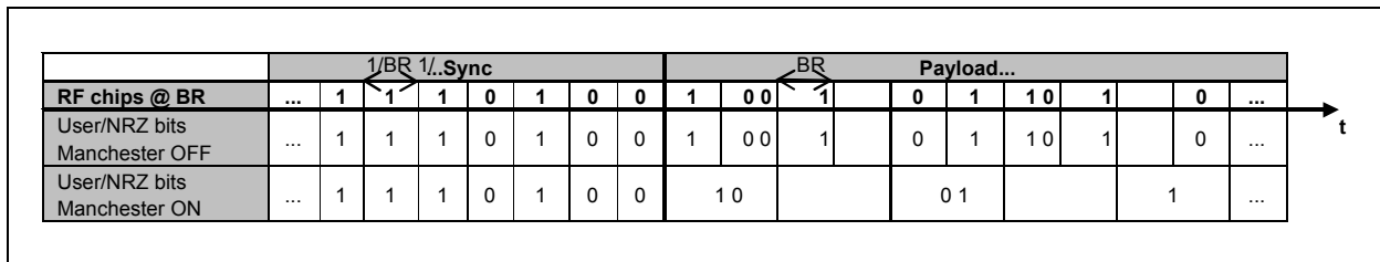
FIGURE 3-30: MANCHESTER ENCODING/DECODING
