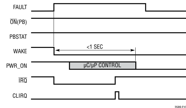
Figure 10. Hard Reset Due to a Fault Condition
