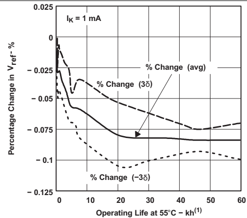
Figure 8. Percentage Change in V_{REF} vs Operating Life at 55°C
