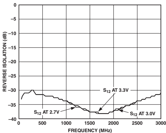
TPC 3. Reverse Isolation vs. Frequency, V_S = 2.7\text{ V} , 3\text{ V} , and 3.3\text{ V} , T_A = 25^\circ\text{C}
