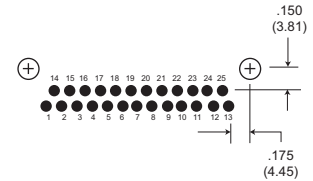
25 Contacts
