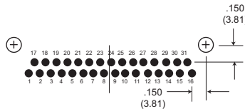
31 Contacts
