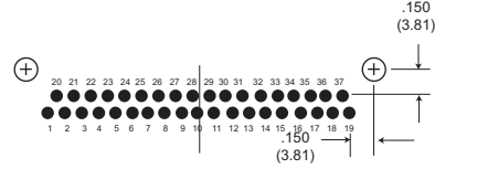
37 Contacts
