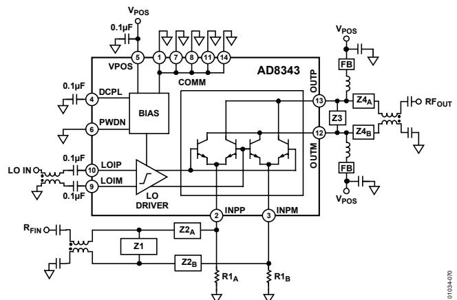
Figure 70. Typical Upconversion Application
