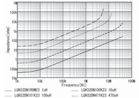
Impedance-Frequency Characteristics (Typ.)
