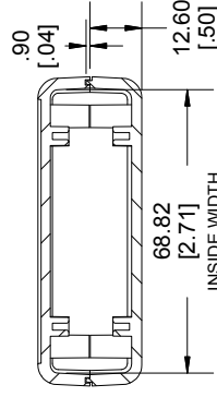
SECTION A-A END VIEW
