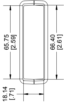
END VIEW
