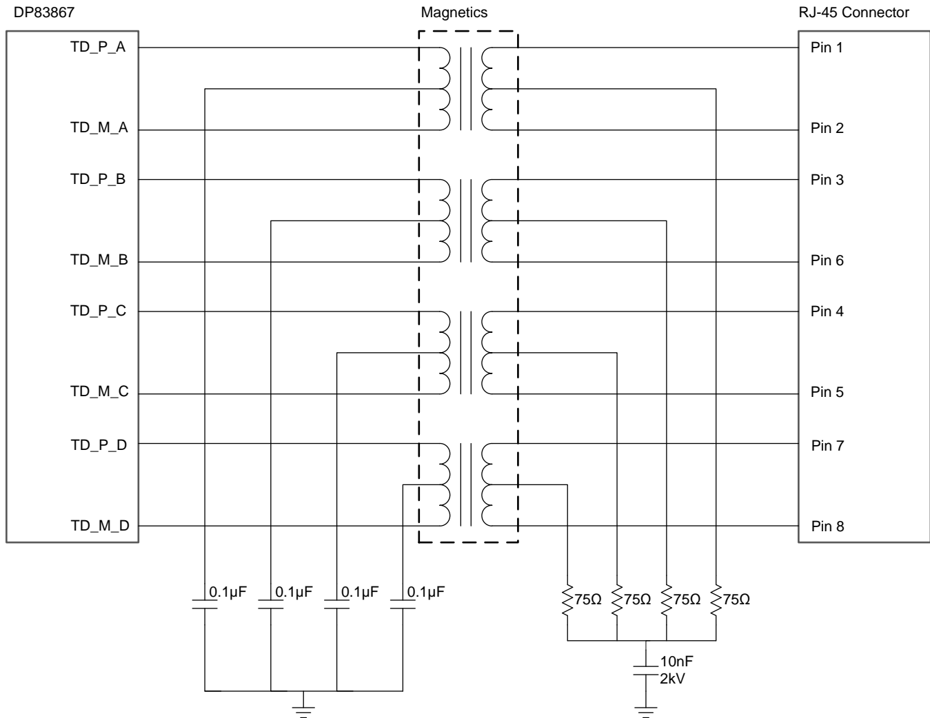
Figure 26. Magnetics Connections
