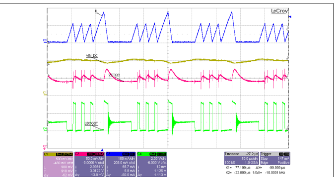
V_{IN\_DC} = sourcemeter with V_{SOURCE} = 2.0\text{ V} and compliance of 43\text{ mA} V_{BAT} = sourcemeter with V_{SOURCE} = 3.0\text{ V} and compliance of 1\text{ A} I_L = inductor current
