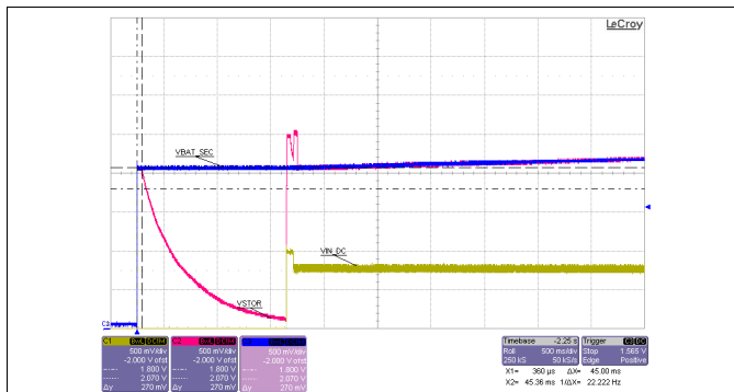
Sourcemeter with V_{SOURCE} = 1.0\text{ V} and compliance of 8.5\text{ mA} subsequently applied to V_{IN\_DC} V_{BAT} = 0.1\text{ F} capacitor charged to 2.0\text{ V} Resistance on V_{STOR} = 100\text{ k}\Omega
