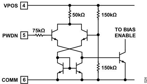
Figure 24. Power-Down Threshold Circuitry
