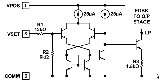
Figure 28. Setpoint Interface Circuitry
