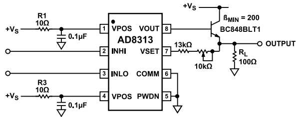
Figure 41. Output Current Drive Boost Connection
