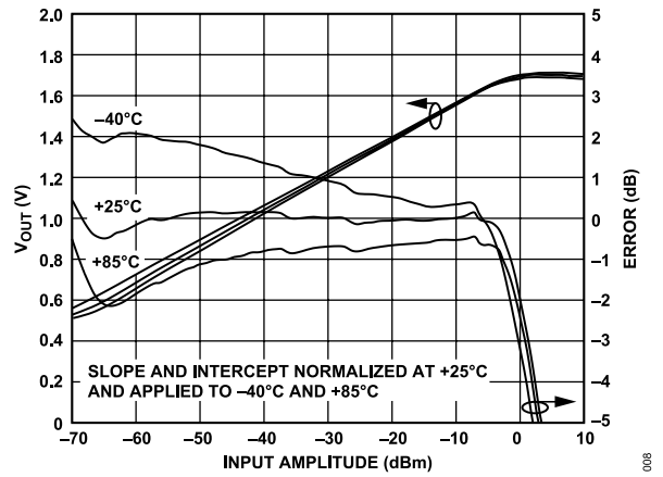
Figure 8. V_{OUT} and Log Conformance vs. Input Amplitude at 1.9 GHz for Multiple Temperatures
