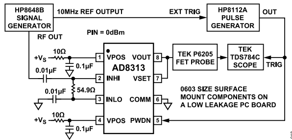
Figure 18. Test Setup for PWDN Response Time
