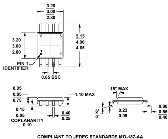
Figure 46. . 8-Lead Mini Small Outline Package [MSOP] (RM-8) Dimensions shown in millimeters
