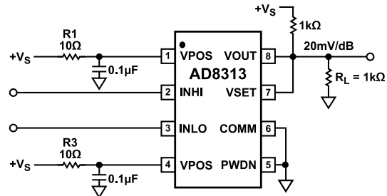
Figure 40. Increasing AD8313 Output Current Capability
