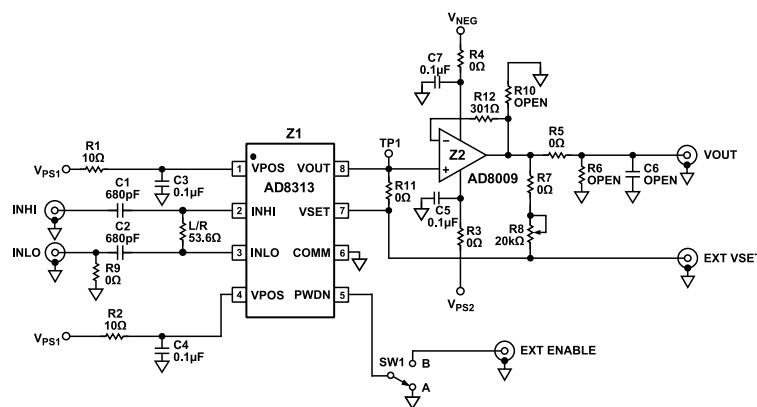
Figure 44. Evaluation Board Schematic
