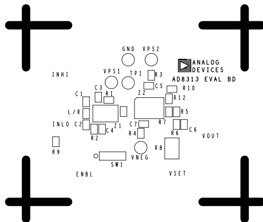
Figure 43. Signal Layer Silkscreen
