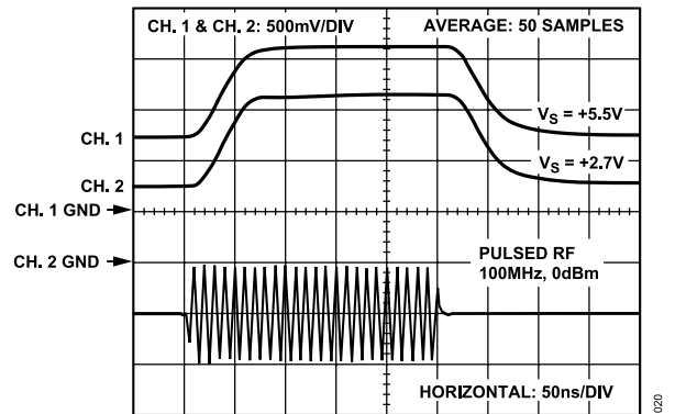
Figure 20. Response Time, No Signal to 0 dBm
