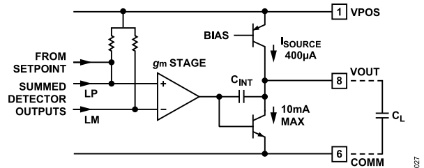
Figure 27. Output Interface Circuitry
