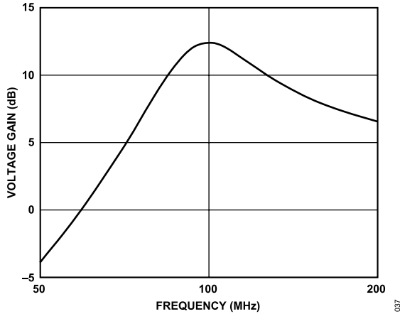
Figure 37. Voltage Response of 100 MHz Narrow-Band Matching Network
