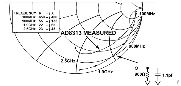
Figure 26. Typical Input Impedance
