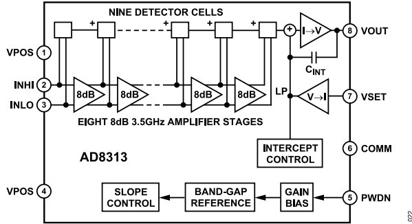
Figure 22. Block Diagram
