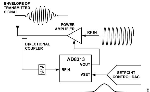
Figure 31. Setpoint Controller Operation
