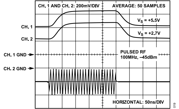
Figure 19. Response Time, No Signal to -45 dBm
