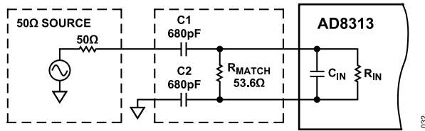
Figure 32. A Simple Broadband Resistive Input Termination
