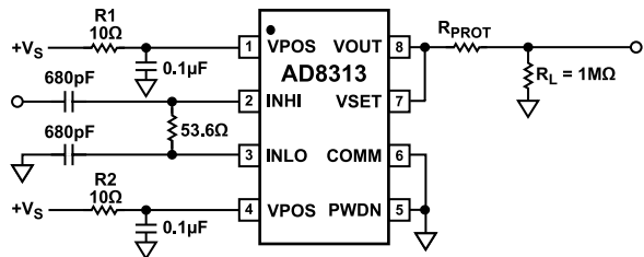
Figure 29. Basic Connections for Log (RSSI) Mode
