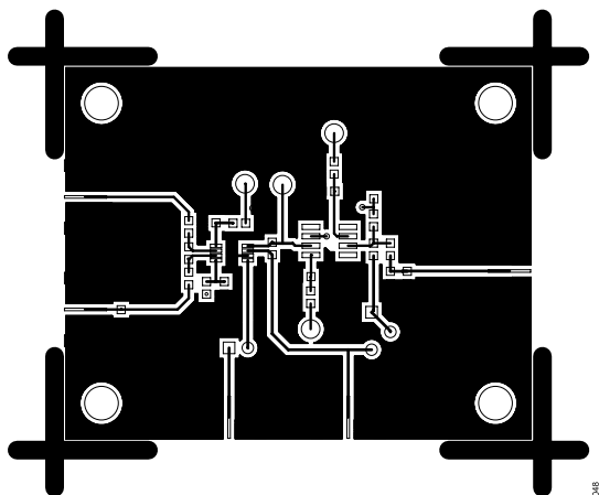
Figure 42. Layout of Signal Layer
