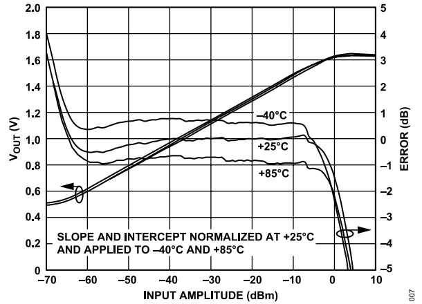
Figure 7. V_{OUT} and Log Conformance vs. Input Amplitude at 900 MHz for Multiple Temperatures
