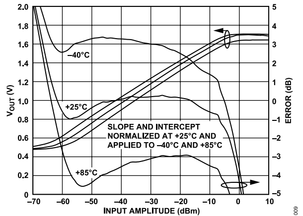
Figure 9. V_{OUT} and Log Conformance vs. Input Amplitude at 2.5 GHz for Multiple Temperatures
