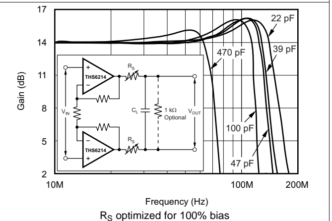
Figure 61. Frequency Response vs Capacitive Load
