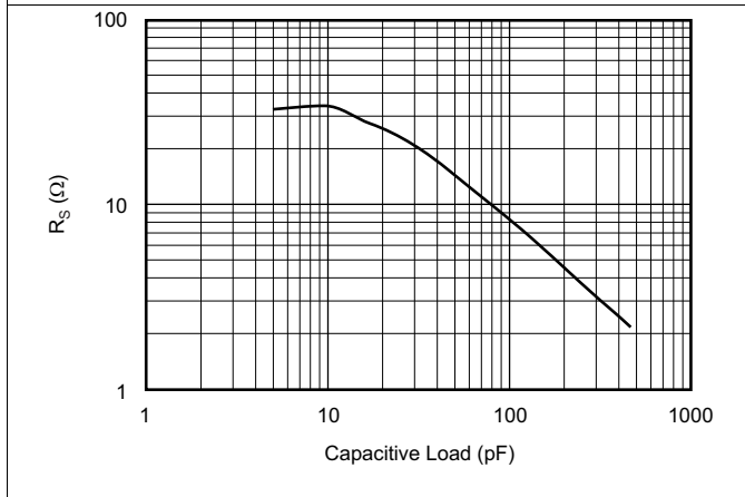
Figure 60. Recommended R_S vs Capacitive Load
