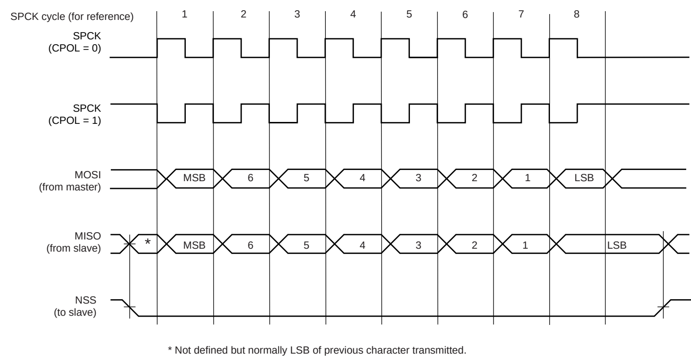
Figure 28-4. SPI Transfer Format (NCPHA = 0, 8 bits per transfer)
