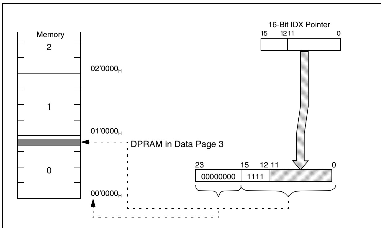
Figure 2-17 Arithmetic MAC Operations and Addressing via the IDX Pointers
