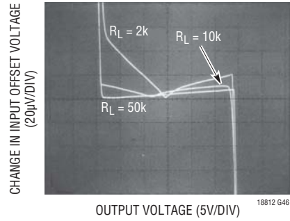
Open-Loop Gain
