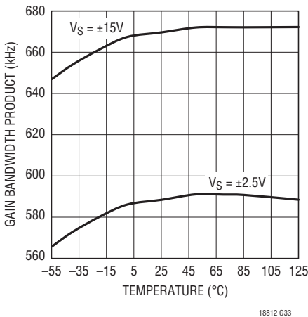
Gain Bandwidth Product vs Temperature
