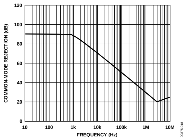
Figure 18. Common-Mode Rejection vs. Frequency
