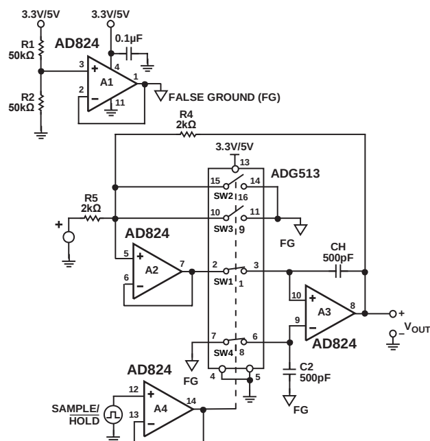
Figure 37. 3.3 V/5.5 V Precision Sample-and-Hold Circuit
