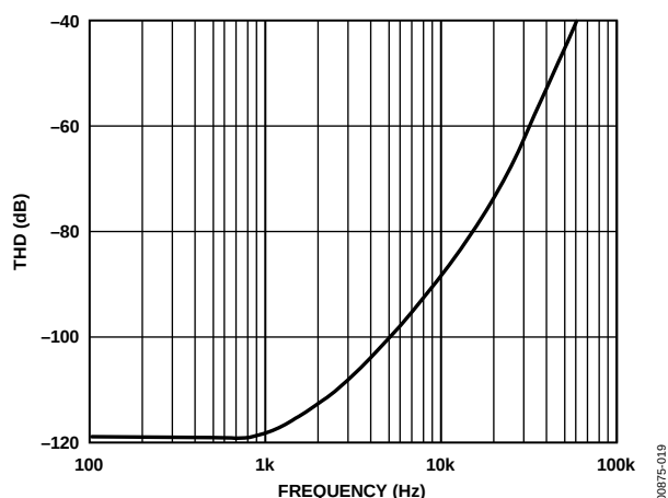
Figure 19. THD vs. Frequency, 3 V rms
