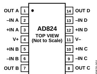
Figure 1. 14-Lead SOIC (R Suffix)
