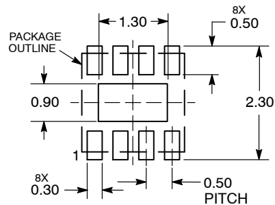
DIMENSIONS: MILLIMETERS
