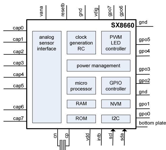
Figure 3 Simplified block diagram of the SX8660
