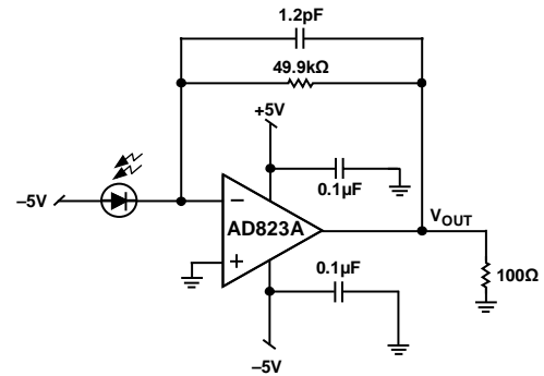
Figure 44. Photodiode Preamplifier
