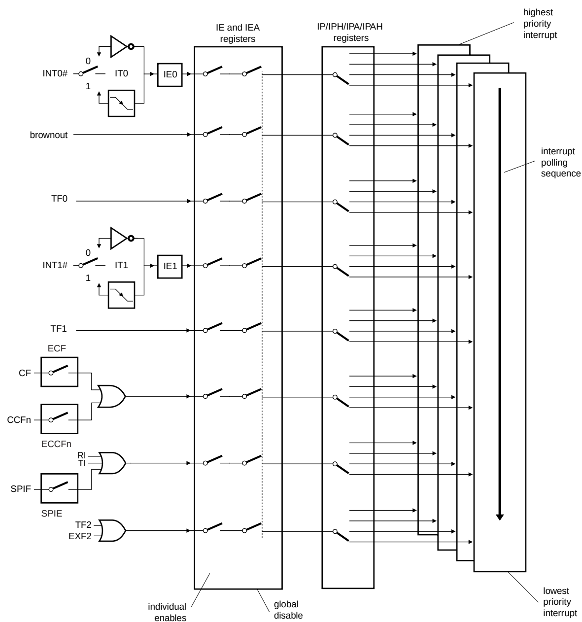
Fig 27. Interrupt structure
